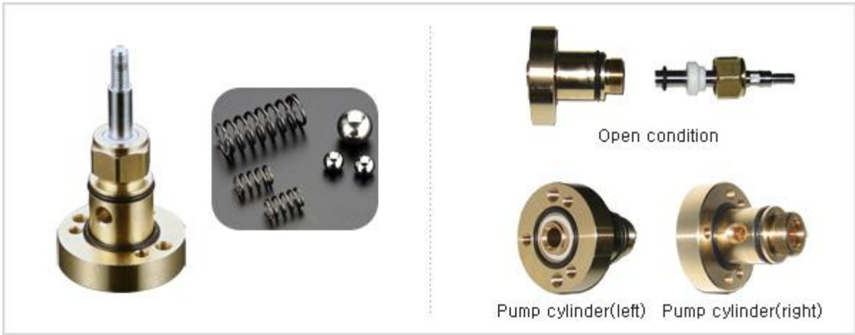
> Cylinder set (ball, spring within)
